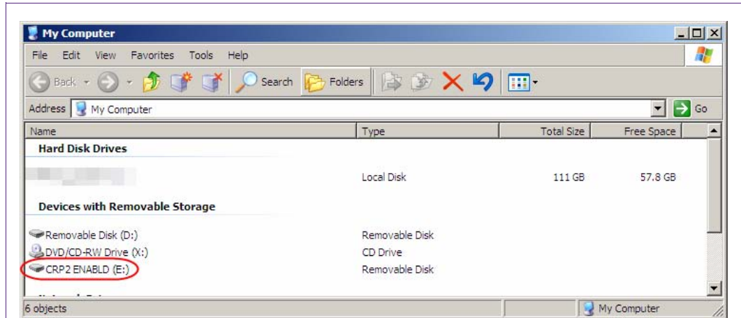
Fig 3. LPC1343 with CRP2 enabled (USB based ISP mode)
