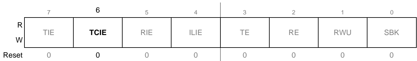
Figure 0-1. SCI Control Register 2 (SCIC2)
