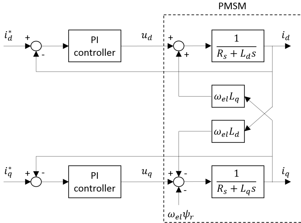
Figure 2-1. The d-q PMSM model
