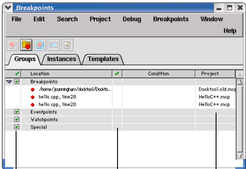
Figure 18.1 Breakpoints Window
