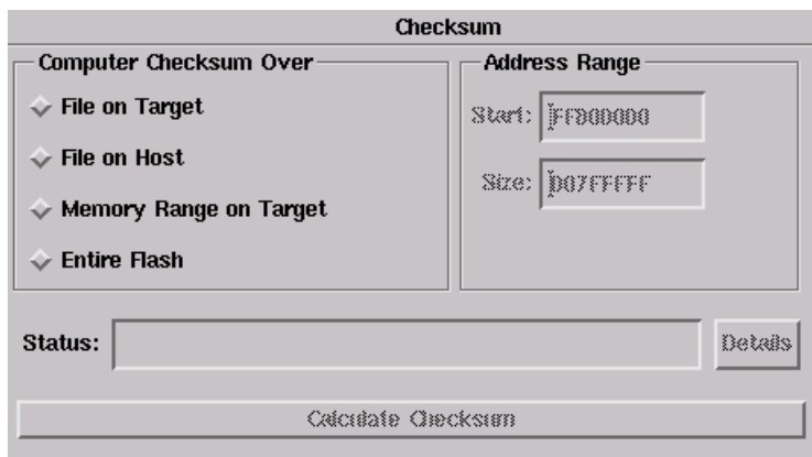
Figure 22.6 Checksum Panel
