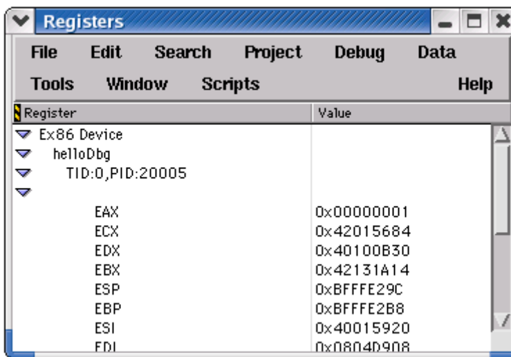
Figure 20.3 Registers Window
