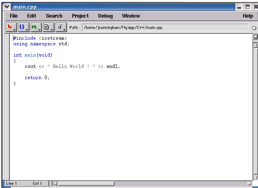
Figure 9.1 Editor Window
