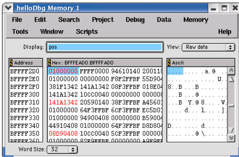
Figure 20.1 Memory Window
