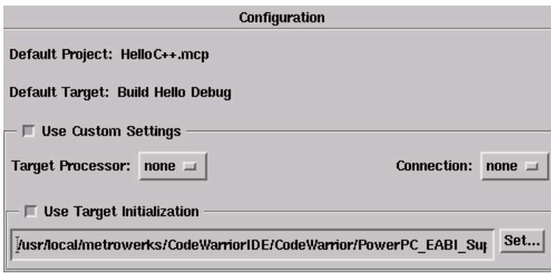
Figure 22.8 Configuration Panel
