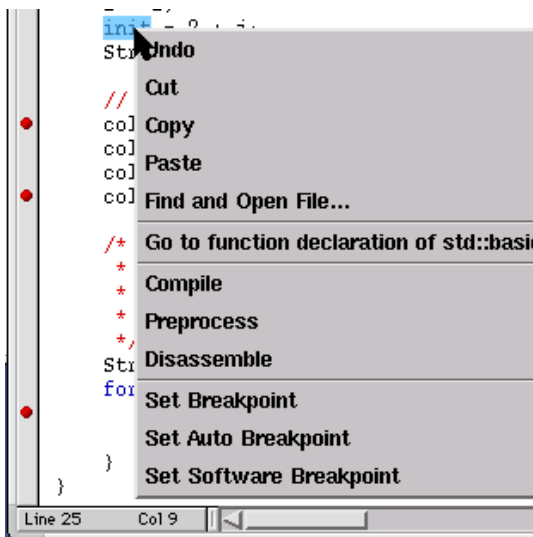
Figure 17.3 Contextual menus
