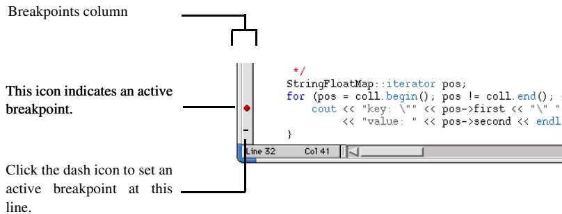
Figure 18.2 Setting Breakpoints
