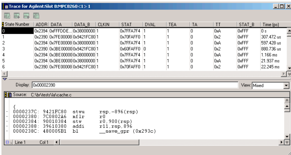
Figure 22.14 Trace Window
