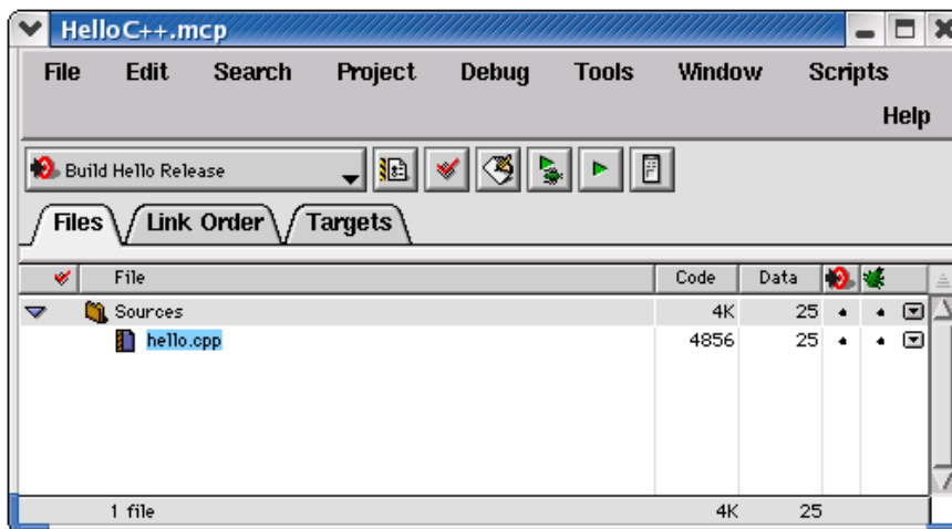
Figure 4.1 Project Window
