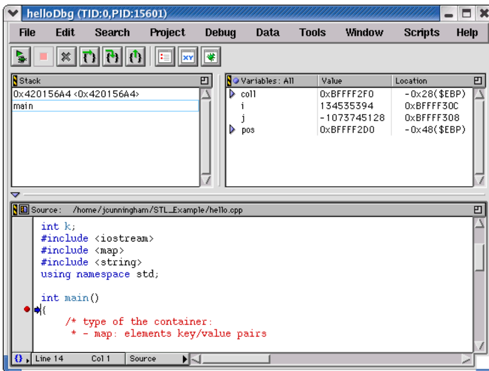
Figure 17.1 Thread Window
