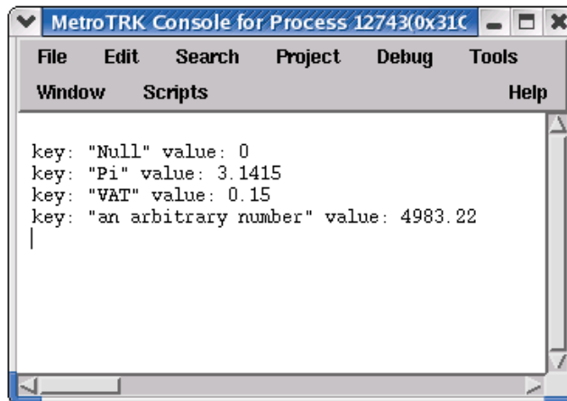
Figure 21.3 Log Window
