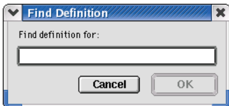
Figure 11.2 Find Definition
